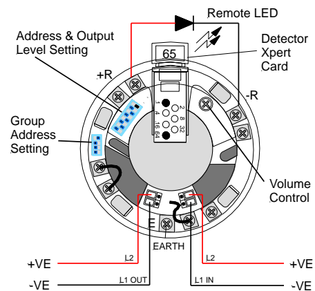
Figure 2: Integrated Base Loop Sounder
