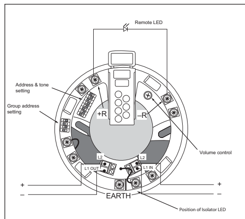
Fig. 2 Sounder Visual Indicator Base with isolator wiring
