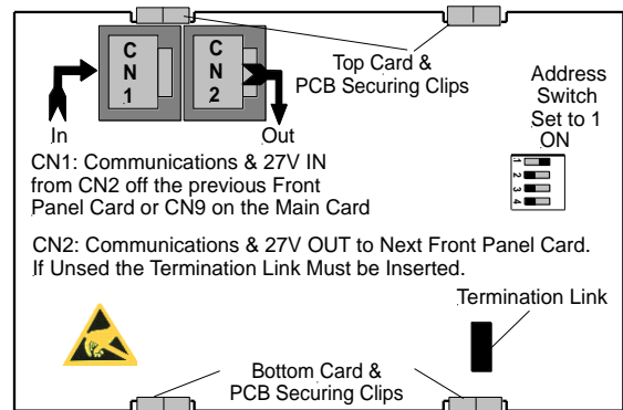
Figure 2: Switch & Indicator Card PCB Layout
