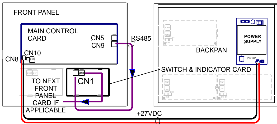
Figure 3: Typical Switch and Indicator Card Cabling to the Main Control Card
