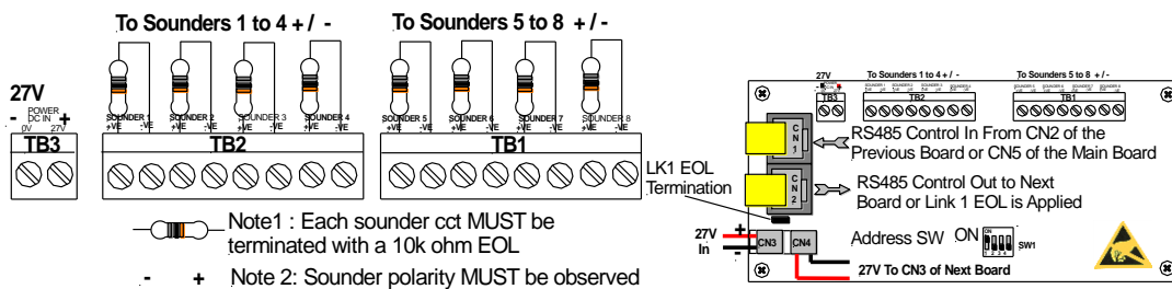
Figure 1: Sounder Board Outputs
