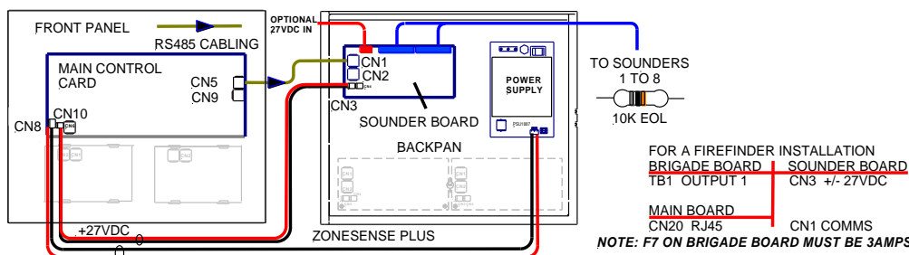
Figure 2: Internal Cabling of the FACP
