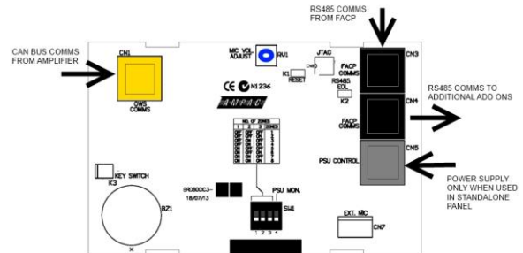
Figure 2: OWS Control Module PCB Layout
