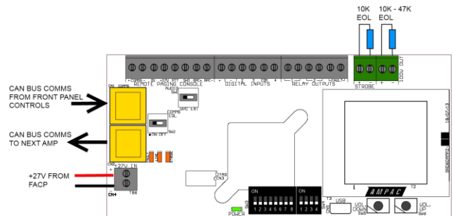
Figure 3: Amplifier PCB Layout
