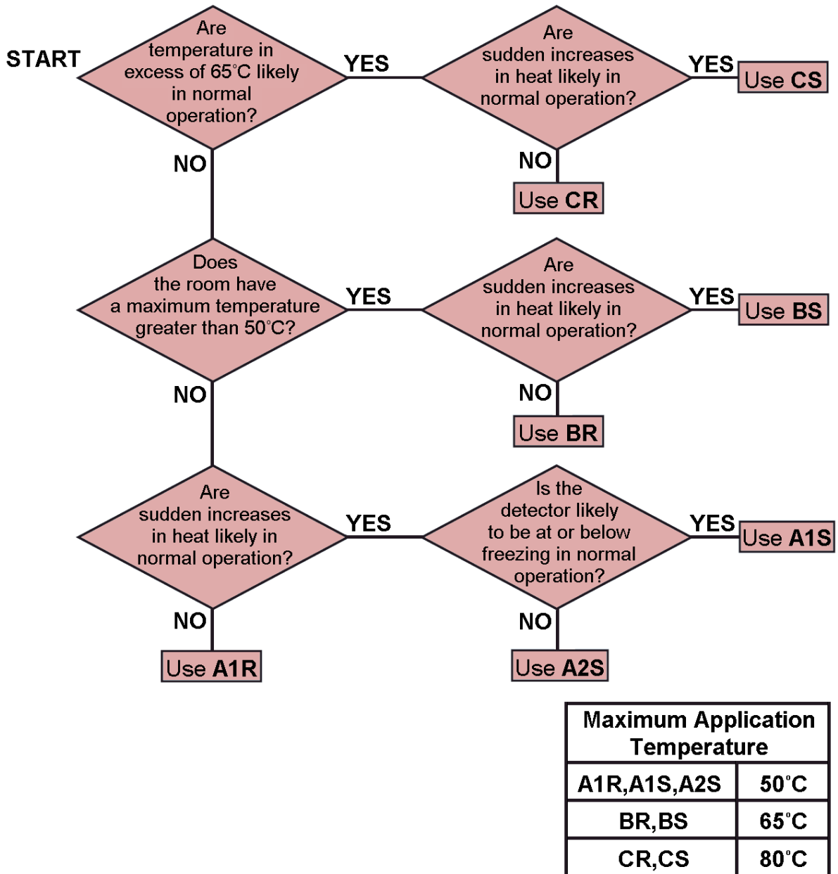
Figure 3 – Choosing a Heat Detector
