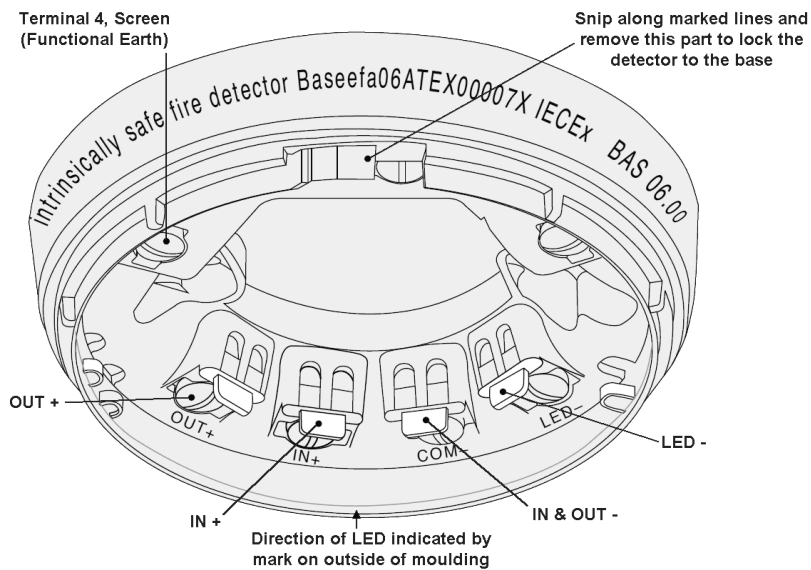
Figure 4 – TimeSaver IS Base
