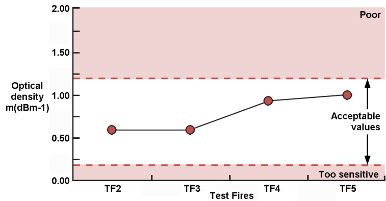
Figure 1 - Orbis Optical Detector Response to Test Fires
