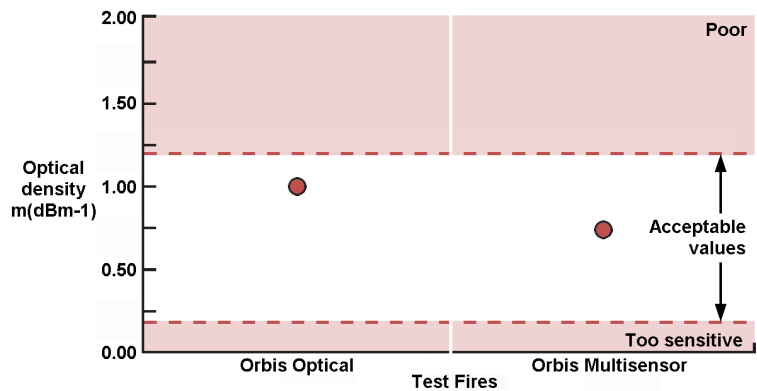
Figure 2 - Comparisons of Response between Orbis Optical & Multisensor
