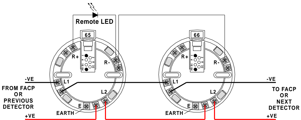
Figure 2: General Wiring Diagram c/w Common Remote LED
