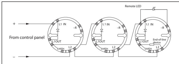
Wiring Diagram of Series 65 Monitored Detector Circuit
