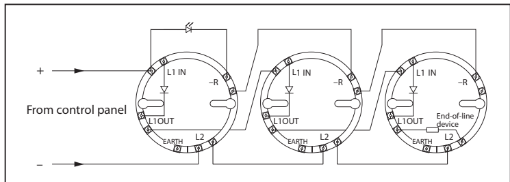
Wiring Diagram of Series 65 Monitored Detector Circuit with a common Remote Indicator
